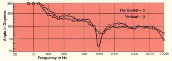
Figure 2. Beamwidth (-6dB) vs. Frequency (4430)
