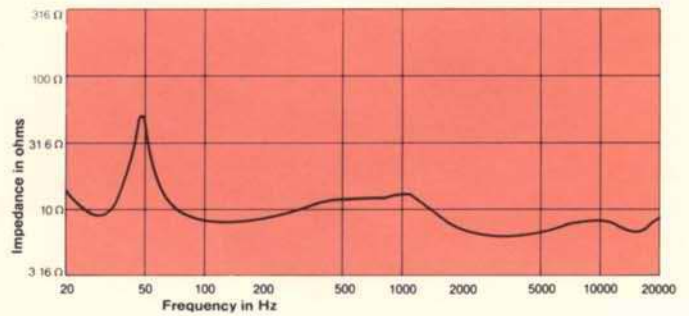
Figure 9. Impedance (4430)
