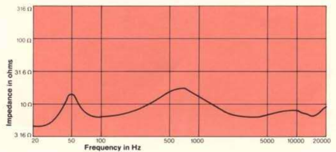
Figure 10. Impedance (4435)
