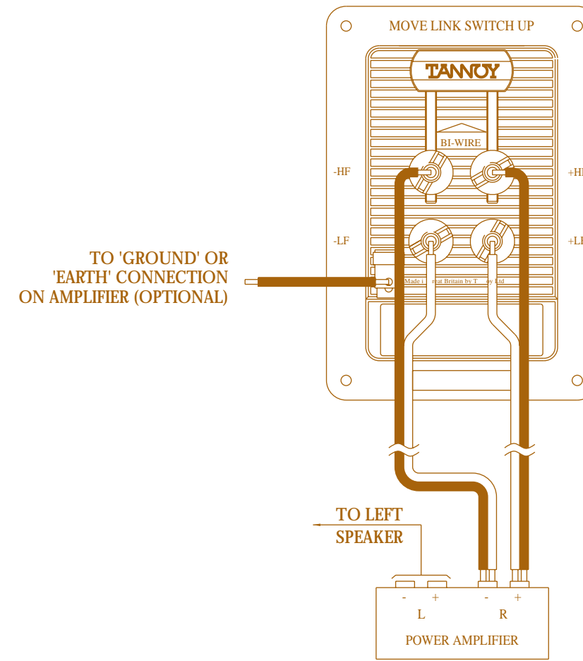
FIGURE 3: Bi-Wire Mode and Earth (Ground) Lead Connection
