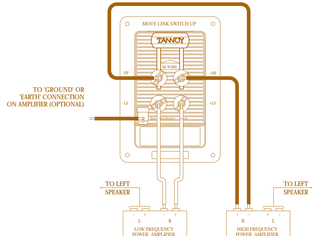
FIGURE 4: Bi-Amping Mode and Earth (Ground) Lead Connection
