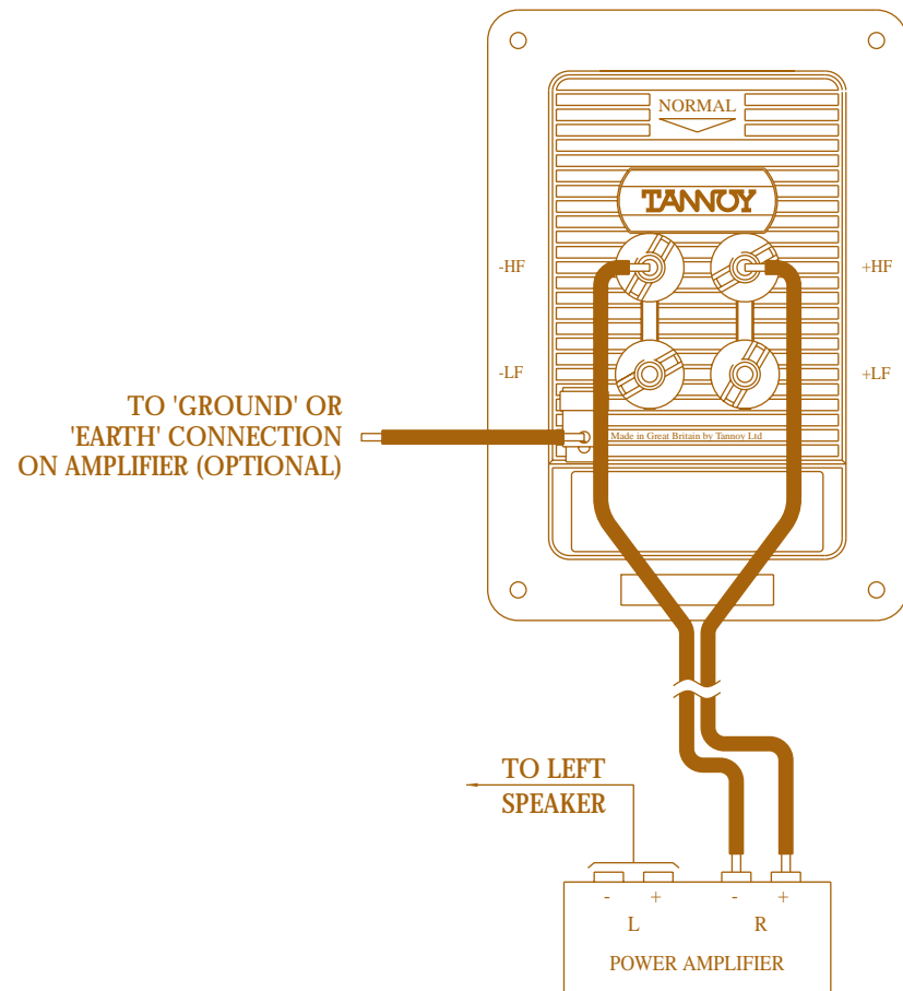
FIGURE 2: Single Wire Mode and Earth (Ground) Lead Connection
