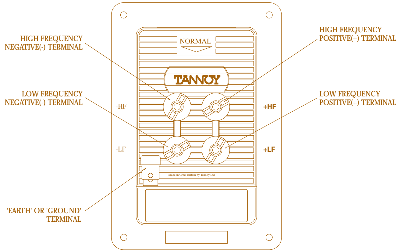
FIGURE 1: Terminal Panel Connections
